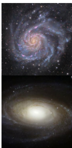
Top: Galaxy M101, an example of a 'flat' galaxy. Bottom: Galaxy M81, an example of a 'fat' bulgy galaxy.
