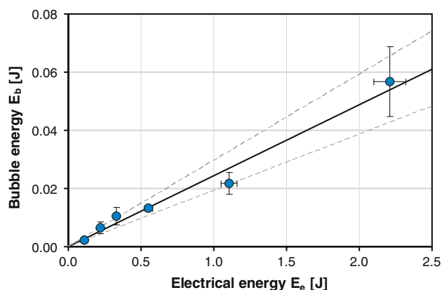
Fig. 8 Mean bubble energy as a function of capacitors electrostatic energy. Solid line : weighted linear regression. Dashed line : regression uncertainties
