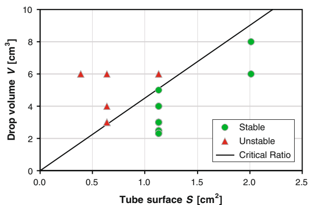
Fig. 3 Diagram representing the different pairs ( V , S ) of drop volume V and tube contact surface S used in the course of the experiment
