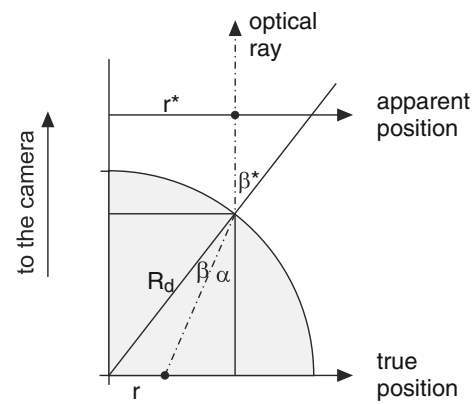
Fig. 11 Model of optical refraction by a spherical drop. Gray zone: quarter of the drop’s cross-section. Dashed-dot line: optical ray
