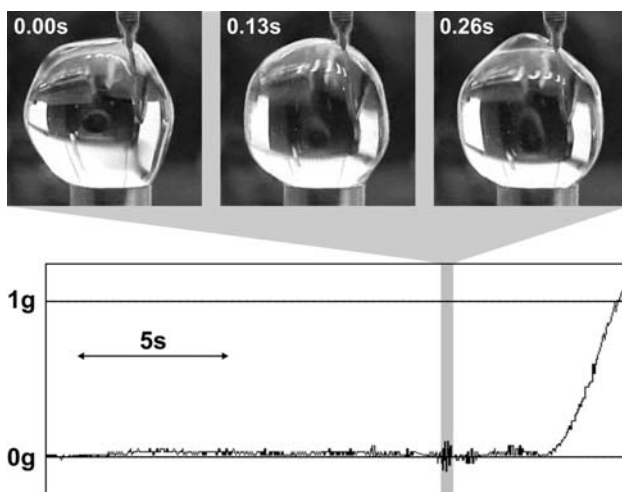
Fig. 2 Top : water drop oscillations resulting from g-jitter superior to 0.05 g, as filmed by the standard video camera (Sect. 3.1). Bottom : vertical component of the acceleration vector versus time
