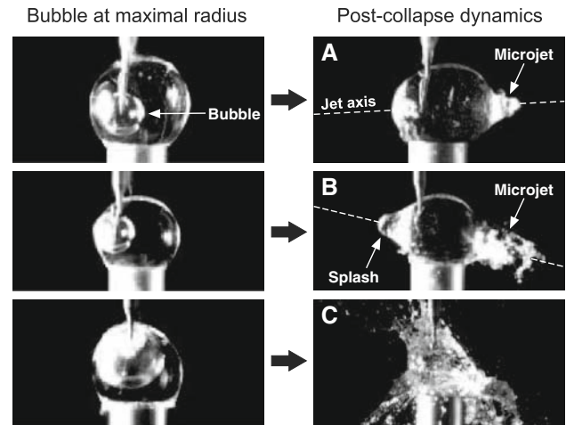
Fig. 9 Three qualitative categories characterizing the strength of jets emission and the stability of the water drop and its surface after bubble collapse. Left column : instant of maximum bubble size, illustrating the relative bubble radius and its position within the drop. Right column : situation 4 ms after, illustrating the three post-collapse dynamics categories. Cat. A: the microjet escapes but the splash does not. Cat. B: the splash escapes and the microjet is more violent. Cat. C: the entire drop bursts
