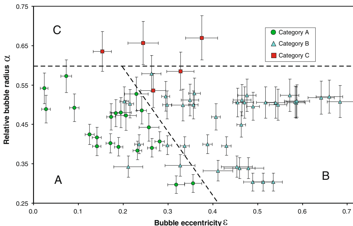
Fig. 10 Representation of 67 parabolas in the parameter space (bubble eccentricity \varepsilon , relative bubble radius \alpha ). The parabola points ( \varepsilon, \alpha ) belonging to different categories A, B, C (introduced in Fig. 9) were plotted with different symbols, in order to identify associated parameter space domains. Straight lines roughly delimiting these
