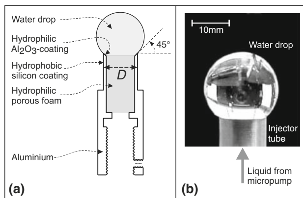
Fig. 1 a Vertical cross section of the injector tube. b Quasi-spherical drop in microgravity
